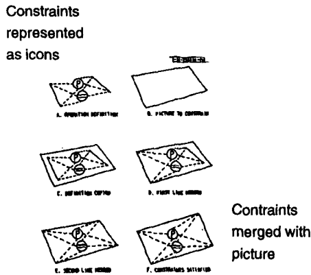
FIGURE 11.5 Programming with constraints
