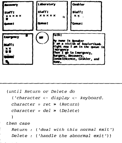
FIGURE 11.41 “Simpula” hospital simulation
